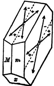
Fig. 817, rhombic section in albite. Fig. 818, same in anorthite. Fig. 819, typical form showing + and - extinction-directions on c(001) and b(010) .
